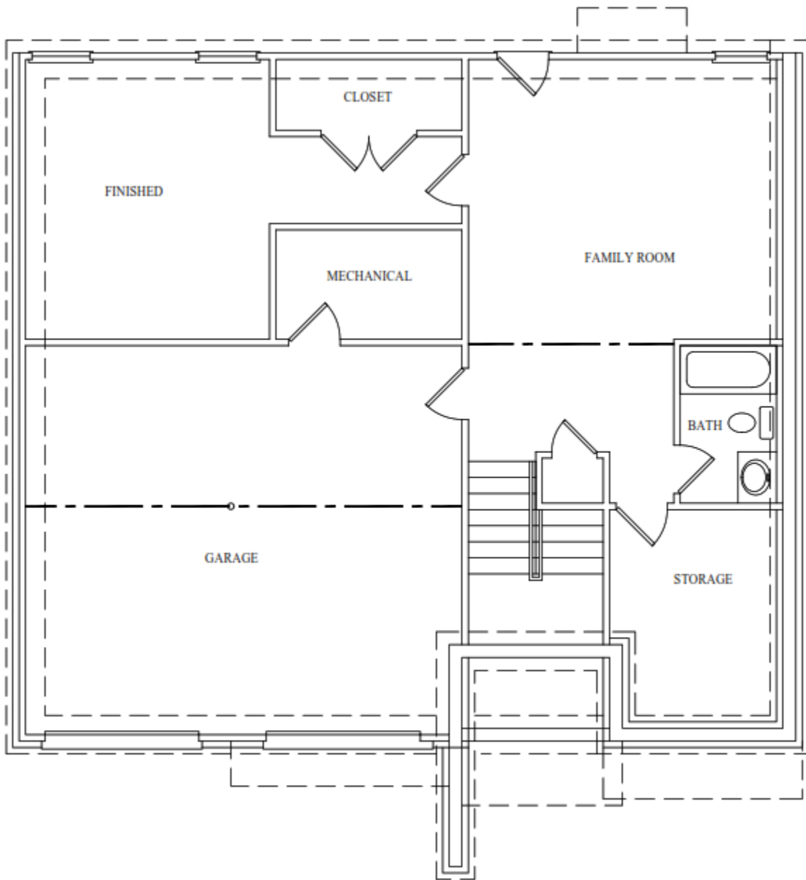
LOWER LEVEL PLAN
